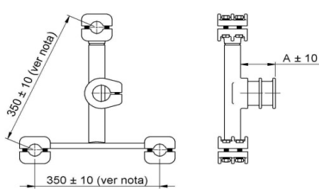
MY3PCC 230 kV
