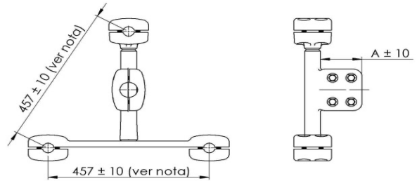
MX3PCC 345 - 550 kV
